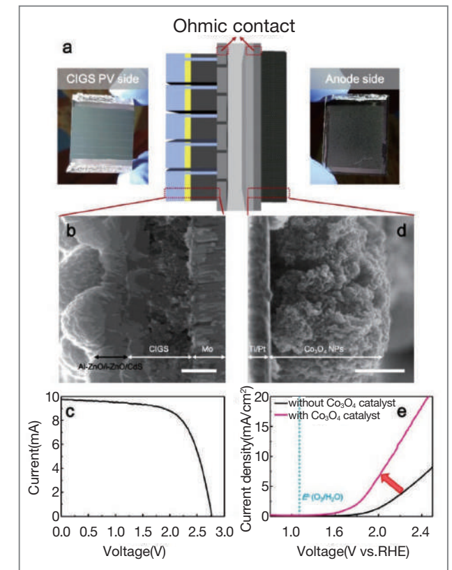
Figure 2. Monolithic CIGS module and \text{Co}_3\text{O}_4 anodic catalyst for photoelectrode. (a) Schematic diagram and photograph of a monolithically stacked photoelectrode with a CIGS PV module and \text{Co}_3\text{O}_4 film on each side of the glass substrate. (b) Cross-sectional SEM image of a CIGS PV cell (scale bar is 1\mu\text{m} ). (c) Typical I-V characteristic of a CIGS module. (d) Cross-sectional SEM image of \text{Co}_3\text{O}_4 film on the glass/Ti/Pt substrate (scale bar is 1\mu\text{m} ). (e) Typical J-V characteristic with and without \text{Co}_3\text{O}_4 catalyst films.
