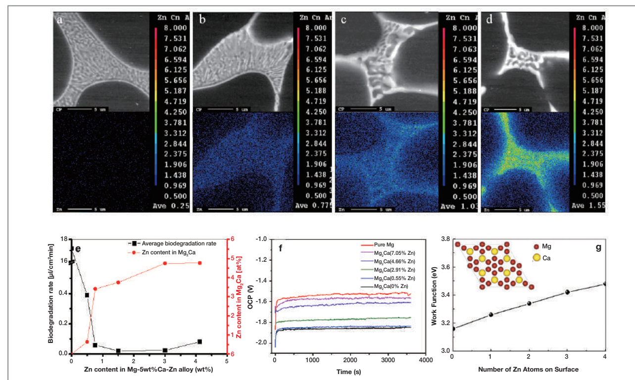
Figure 2. a–d. SEM and the corresponding WDS images showing the distribution of dissolved Zn in Mg-5wt%Ca-xwt%Zn alloys (x = 0, 0.5, 1.0, and 1.5 from the left). e. Relationship between the biodegradation rate of Mg-Ca-Zn alloys and the Zn concentration inside Mg 2 Ca obtained from WDS analysis. f. Measurement of the open-circuit potential (OCP) of the immersed Mg 2 Ca alloys with various Zn concentrations. g. Variation of the work function with Zn contents in the (0001) surface of Mg 2 Ca (Inset. Atomic configuration of the (0001) surface where red spheres represent Mg atom and gold spheres represent Ca atom).
