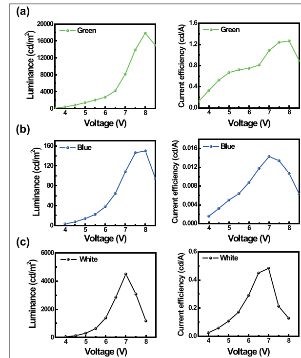
Figure 6. Luminance versus voltage and current efficiency versus voltage characteristics of (a) green, (b) blue, and (c) white QDLEDs.
