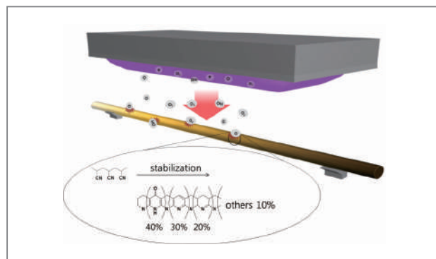
Figure 5. Scheme of plasma-assisted stabilization process [14].
