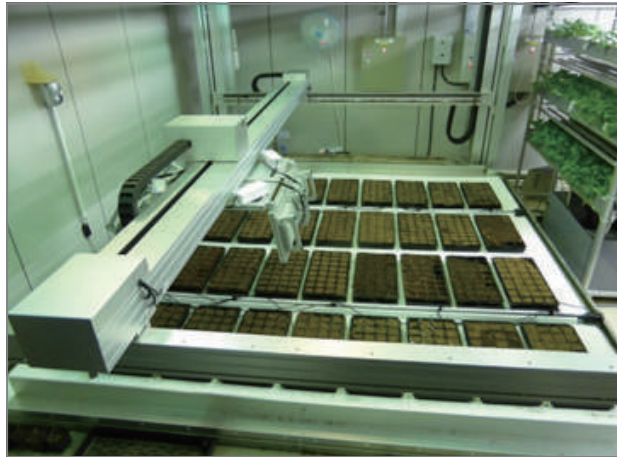
Figure 4. KIST's custom built sensor-to-plant type plant phenotyping platform.
