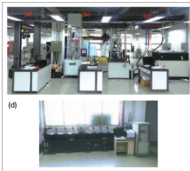
Figure 9. Specialized equipments at KIST Jeonbuk. (a) High-load tensile tester. (b) Fatigue testing system. (c) High-performance shock tester. (d) Hopkinson bar tester.
