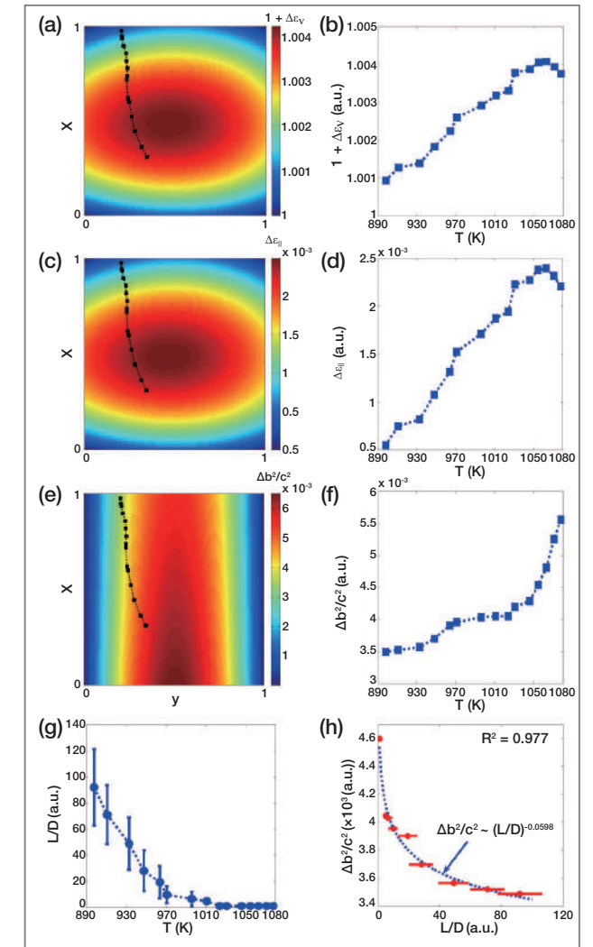
Figure 4. (a) 2D map for the variations of the volumetric ratio between the concentration-weighted summation of unit cell volumes of HWZ CdS, CdSe, ZnS, and ZnSe and the unit cell volume of HWZ alloy Cd_{0.78}Zn_{0.22}S_{0.23}Se_{0.77} ( 1 + \Delta\epsilon_v ) as a function of x and y . In the map, black circles are the composition data extracted from the observed alloy nanostructures. (b) Dependence of 1 + \Delta\epsilon_v as a function of T . (c) As (a), but for the biaxial strain factor \Delta\epsilon_{il} . (d) Dependence of \Delta\epsilon_{il} as a function of T . (e) As (a), but for the bond length mismatch parameter ( \Delta b^2/c^2 ). (f) Dependence of \Delta b^2/c^2 as a function of T . (g) Ratio between the width and thickness of the nano-plate shaped alloy nanostructures ( L/D ) as a function of T . (h) Dependence of ( \Delta b^2/c^2 ) as a function of L/D . The data is fitted with a power-law function such that \Delta b^2/c^2 \sim (L/D)^{\alpha} .
