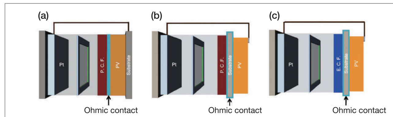
Figure 1. (a) Solar-fuel device with photocatalytic film (P.C.F.) and internal PV. (b) Solar-fuel device with photocatalytic film (P.C.F.) and external PV. (c) Solar-fuel device with electrocatalytic film (E.C.F.) and external PV.
