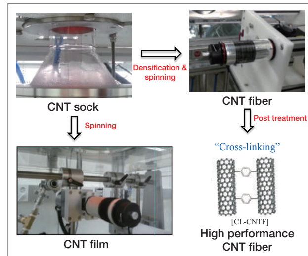
Figure 2. Digital images of CNT socks, CNT fiber, and CNT film synthesized by the direct spinning method. The scheme of high performance CNT fiber produced by introduction of chemical cross-linking between CNT bundles.
