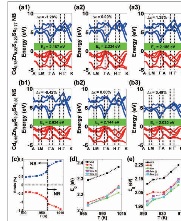
Figure 3. Calculated electronic band structures of the quaternary alloy NBs with different residual strains ( \Delta\epsilon ) and NSs with different residual strains. (c) Dependence of \Delta\epsilon at different T . (d) Dependence of E_g with increasing T . Calculated values of E_g (black dotted lines) are compared with the experimentally observed values (PL (red) and Abs (green) dash-dot lines) and calculated values obtained by the bowing equations with different parameter sets for the alloy NBs with tensile (t, maroon lines) and compressive (c, cyan lines) residual strains, respectively. (e) As (d), but for the alloy NSs.
