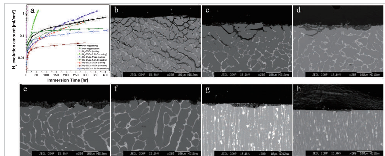
Figure 1. Corrosion and corrosion microstructure measurements of crystalline Mg-Ca-Zn alloys. a. Hydrogen-evolution measurements showing a distinct drop in response to the addition of Zn and by mechanical extrusion. b–f. SEM images of Mg-5wt%Ca-xwt%Zn alloy samples ( x = 0, 0.5, 1.0, 1.5, 3.0 ) after the immersion test in Hank's solution. g, h. SEM images of extruded Mg-5wt%Ca-xwt%Zn alloy samples ( x = 0.5, 1.0 ) after the immersion test in Hank's solution.
