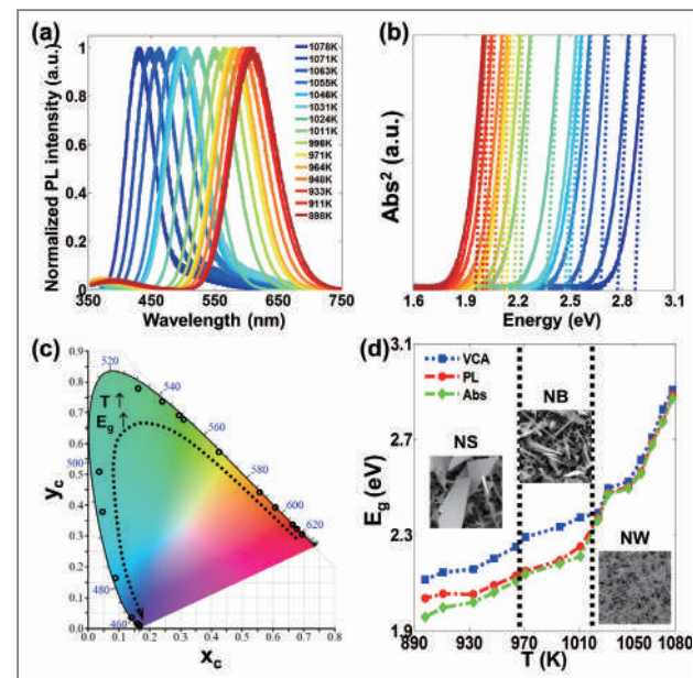
Figure 2. (a) Normalized photoluminescence (PL) and (b) squared UV-Vis absorbance (Abs) spectra of the alloy nanostructures grown at different T . (c) Visible colors from the PL spectra fixed on the CIE-1931 color map. (d) Dependence of E_g as a function of T : expected values from the VCA model (blue marks and dotted line) and experimentally measured values obtained from the PL (red marks and dash-dot lines) and Abs (green marks and dash-dot lines) spectra.
