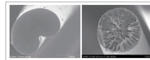
Figure 4. Structures of PAN and mesophase pitch base carbon fibers.
