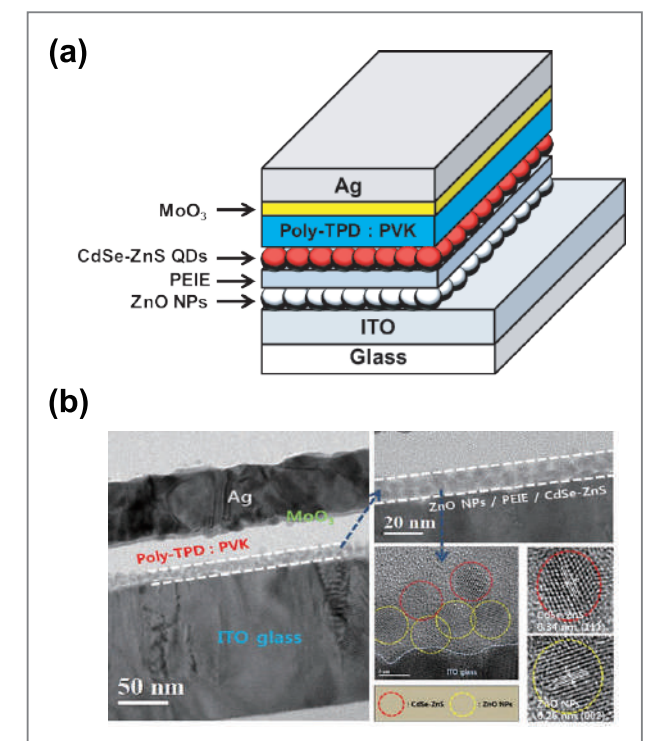
Figure 1. Device structure and TEM images. (a) A schematic cross-sectional view of an inverted red QDLED and (b) corresponding cross-sectional high-resolution transmission electron microscopy (HRTEM) images.
