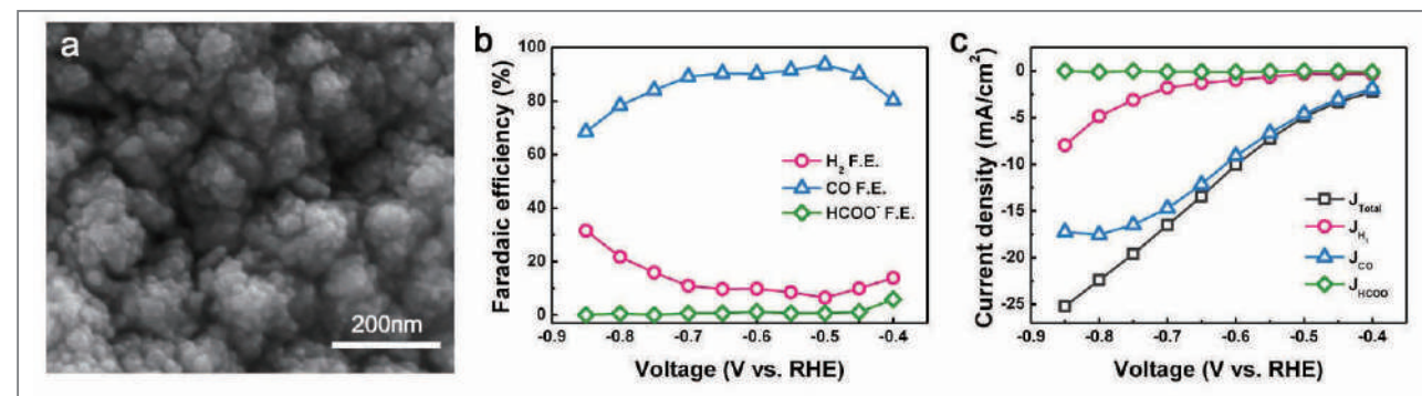
Figure 3. Nanostructured Au for cathodic catalyst. (a) SEM images of nanostructured Au cathodic catalyst. (b) Faradaic efficiency of \text{H}_2 , CO, and formate at varying potential on nanostructured Au cathode for \text{CO}_2 reduction. (c) Total and partial current densities of \text{H}_2 , CO, and formate at varying potential on nanostructured Au cathode for \text{CO}_2 reduction.
