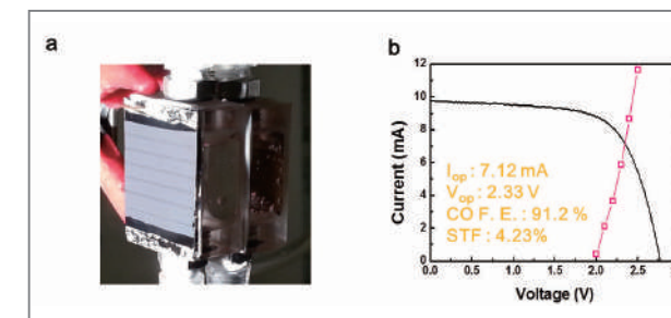
Figure 4. Solar-fuel device performance. (a) Photograph of illuminated solar-fuel device in operation, in which the CIGS module was incorporated at the external side of the PEC cell. (b) The operating point of the solar-fuel device under chopped light illumination.
