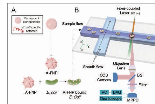
Figure 1. Schematics of the present microbe detection system. (A) Preparation of aptamer conjugated fluorescence nanoparticles (A-FNPs). (B) Detection of A-FNP-bound E. coli by the microchannel and optical particle counter.
