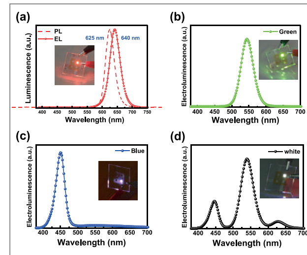
Figure 5. Red, green, blue, and white full color QDLED. (a) Photoluminescence spectrum of CdSe-ZnS QDs solution (dashed line) and electroluminescence spectra (solid line with circle symbol) of red QDLEDs adopting the ZnO NPs/PEIE layer. Electroluminescence spectra of (b) green, (c) blue, and (d) white QDLEDs with ZnO NPs/PEIE layers. Insets show photographs of red, green, blue, and white devices with a ZnO NPs/PEIE layer at applied voltages of 6.5–7.5 V.
