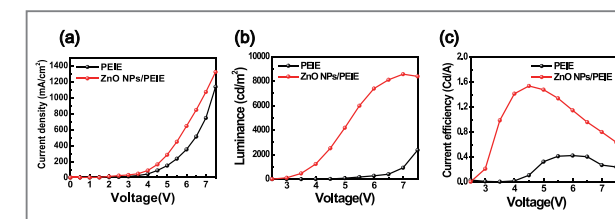
Figure 4. QDLED device characteristics. (a) Current density versus voltage, (b) luminance versus voltage, and (c) current efficiency versus voltage characteristics of QDLEDs with PEIE and ZnO NPs/PEIE layers.
