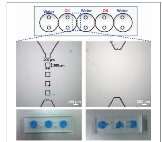
Figure 3. Influence of micro-pillars on the robust interfacial tension of two reagents: blue liquid indicates the water mixed with food dye, and the rest of the chambers contain mineral oil. The water-oil interfaces were maintained better in the presence of pillars as opposed to having no pillars. The pictures were taken immediately after filling the chambers with reagents.
