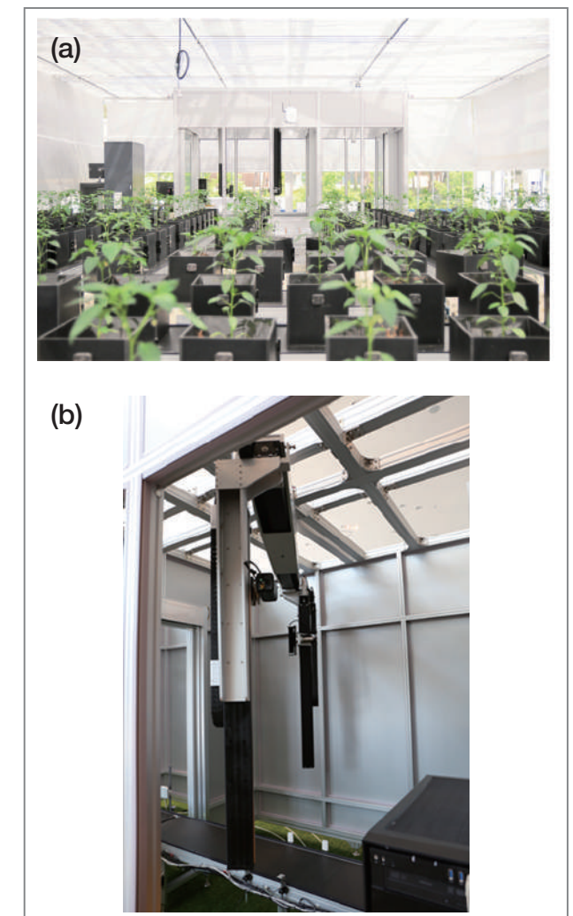
Figure 3. KIST's custom built plant-to-sensor type plant phenotyping platform: (a) layout of the whole system, (b) plant sample moved to the three dimensional (3D) stereo camera to obtain 3D images.
