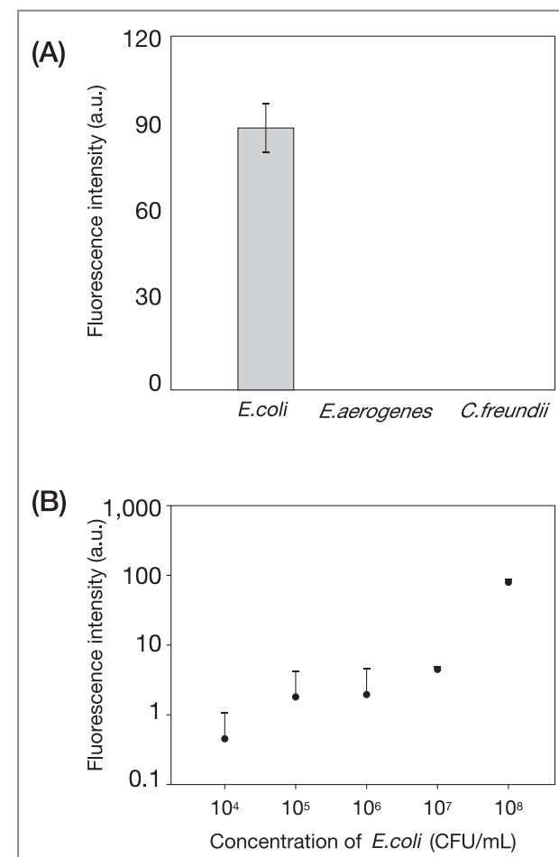
Figure 3. Characterization of A-FNP binding by (A) determining A-FNP selectivity for E. coli and (B) measuring A-FNP binding with increasing E. coli CFUs. (A) A-FNPs bound specifically to E. coli , but not other strains. (B) Fluorescence intensities were dependent upon the number of bacterial cells tested, indicating that A-FNPs can potentially be used for quantitative assays.
