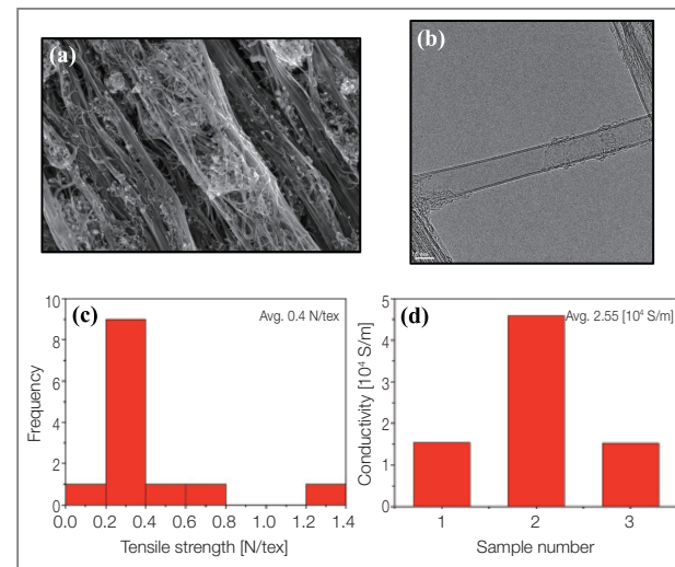
Figure 3. (a) SEM image of CNT fiber and (b) TEM image of a double walled CNT composing CNT fiber. (c) Mechanical and (d) electrical properties of as-synthesized CNT fibers.
