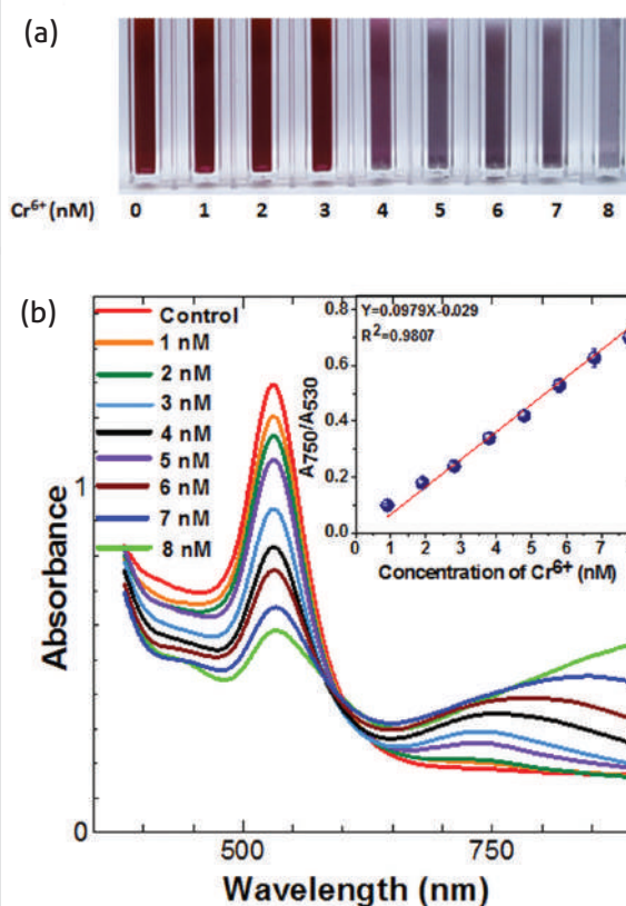
(a) Photographic images of the color change of label-free AuNPs upon addition of \text{Cr}^{6+} ions with various concentrations (0, 1, 2, 3, 4, 5, 6, 7 and 8 nM). (b) UV-vis absorption spectra of label-free AuNPs upon addition of \text{Cr}^{6+} ions with various concentrations (0, 1, 2, 3, 4, 5, 6, 7 and 8 nM).
