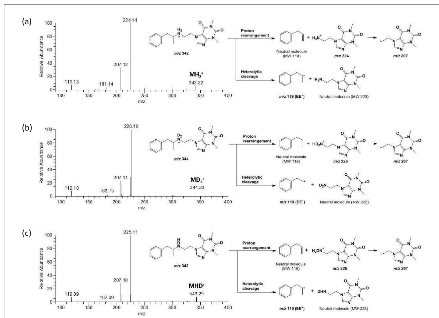
Figure 4 Product ion spectra and fragmentation pathways of (a) unexchanged MH 2 + , (b) fully exchanged MD 2 + , and (c) partially exchanged MHD + ions of fenetylline obtained by GC-ESI/MS-based H/D exchange.
