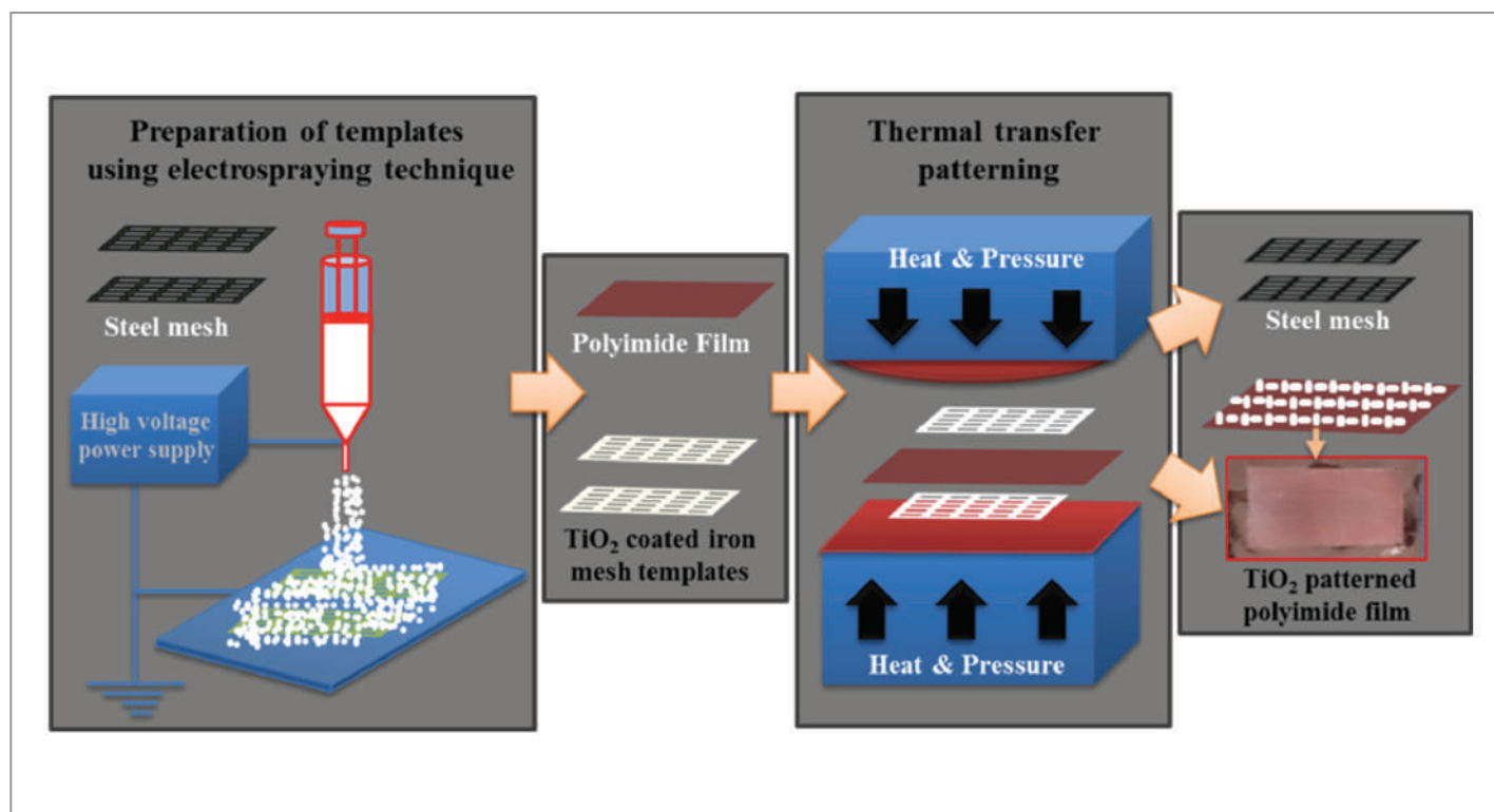
Figure 3 Schematic of experimental procedure for fabricating \text{TiO}_2 -patterned polyimide film.
