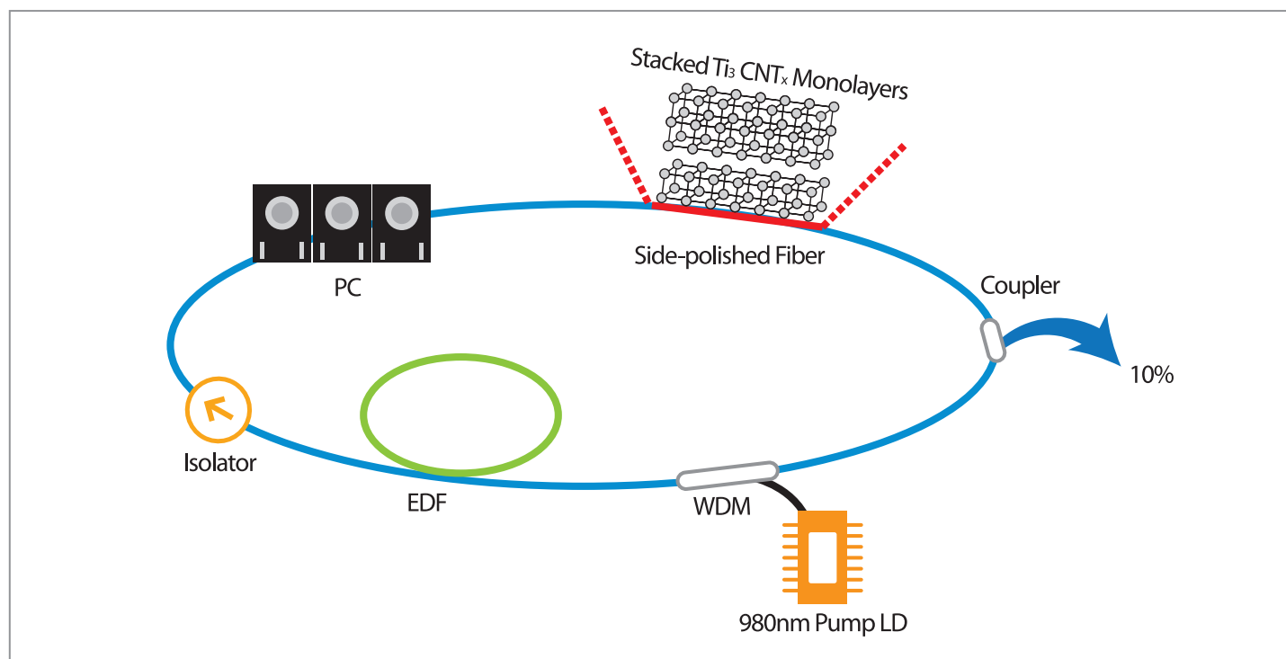
Figure 1 Schematic of the ring-cavity erbium-doped fiber laser incorporating stacked \text{Ti}_3\text{CNT}_x SAs. Here, PC, EDF, WDM, and LD denote a polarization controller, an Er-doped fiber, wavelength division multiplexing, and a laser diode, respectively.
