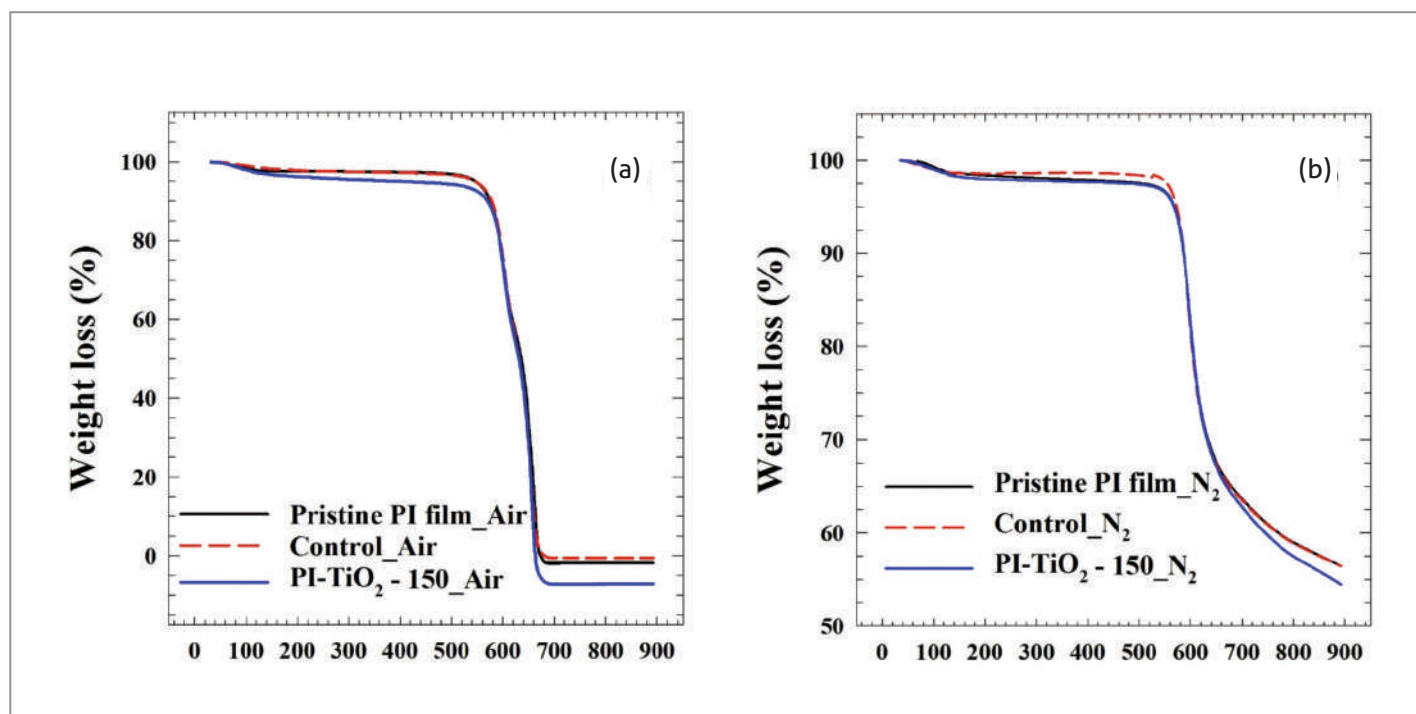
Figure 4 Thermograms of pristine PI, substrate control and PI- \text{TiO}_2 -150 recorded at (a) air and (b) \text{N}_2 atmospheres (scan rate = 10 °C/min).
