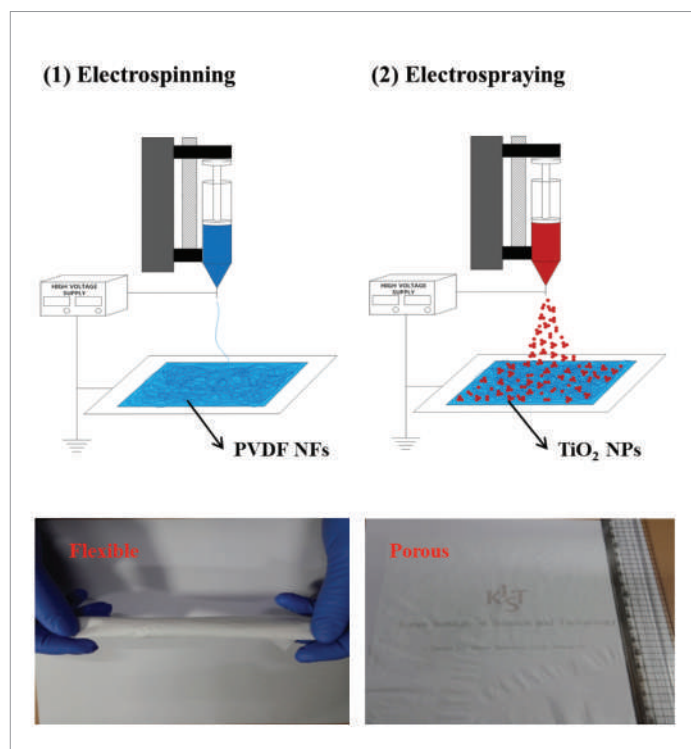
Figure 1 Fabrication of photocatalytic paper (PVDF-TiO 2 hybrids) via electrospinning and electrospraying (adapted from Ramasundaram et al. [3]).
